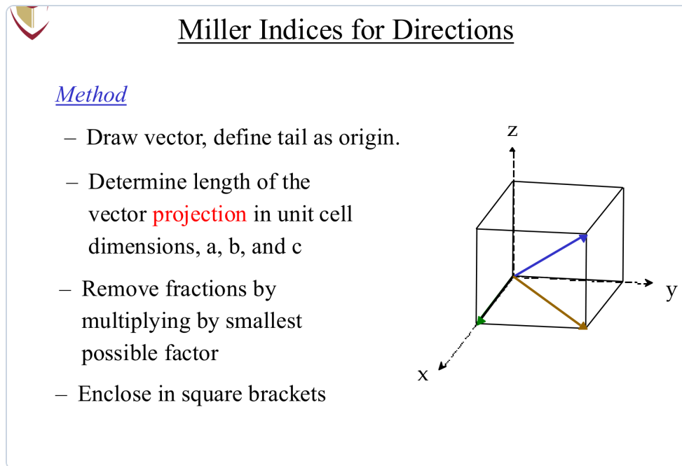
Figure 3.8: Specification of Crystallographic Direction Indices [uvw] (Dr. Medraj Lecture 5). Vector tail is positioned at origin (0, 0, 0) and tip at (x_2, y_2, z_2) . Multiples of a, b, c are reduced to the smallest integers enclosed in square brackets [uvw] . Negative indices are designated with an overbar [\bar{u}vw] .
