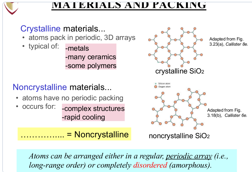
Figure 3.1: Fundamental comparison of atomic arrangements (adapted from Dr. Medraj MIAE 221 Lecture 4 & Callister Fig. 3.23). (a) Crystalline solid exhibiting strict periodic long-range order across macroscopic dimensions (metals, alloys, semiconductors). (b) Amorphous vitreous structure exhibiting short-range chemical bonding without translational lattice periodicity (inorganic silicate glasses, amorphous polymers).
